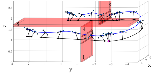
Fig. 3. Maneuvering through window-like obstacles
