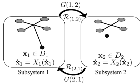
Fig. 1. Quadrotor with a cable-suspended load hybrid system
