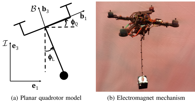
Fig. 5. Quadrotor with cable-suspended load
